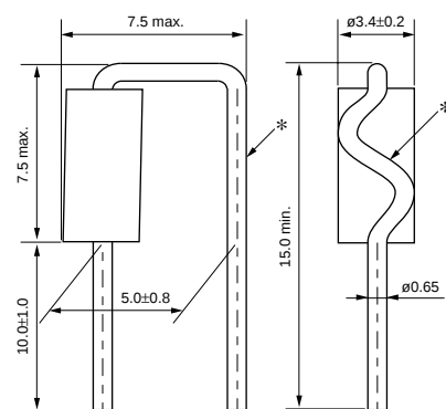
BL02RN1R2M2B
