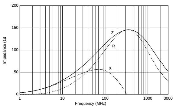
BLM18KG121TN1
