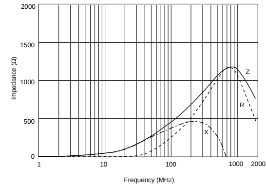
BLM18HD471SN1
