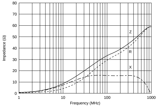
BLM03PG330SN1
