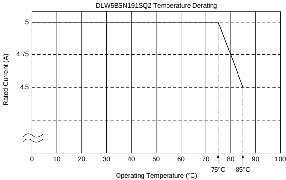
DLW5BSN191
