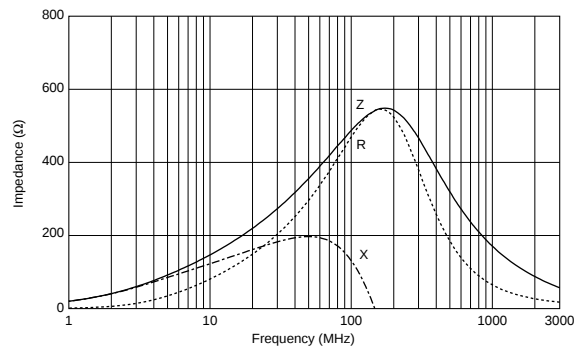
BLM18KG471SN1
