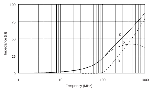
BLA2ABB220SN4
