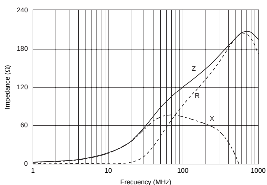
BLM15PD121SN1
