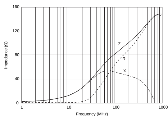
BLM15PD800SN1
