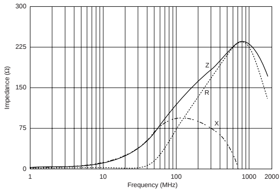
BLA2ABD121SN4
