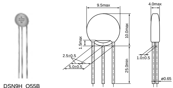
DSN9H_Q55B
