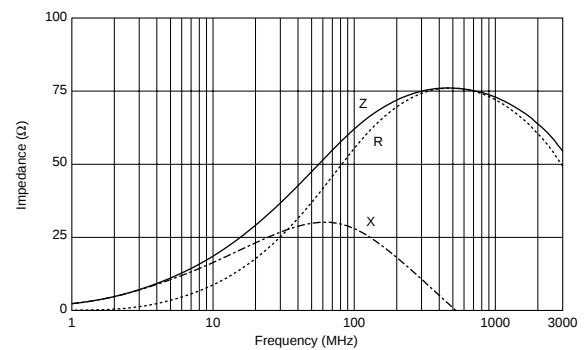
BLM18KG700TN1
