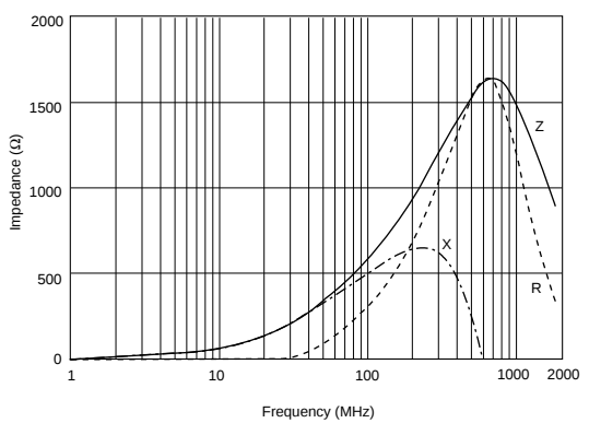
BLM18HD601SN1
