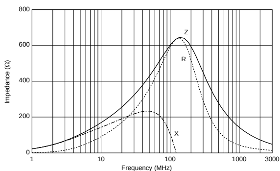
BLM18KG601SN1
