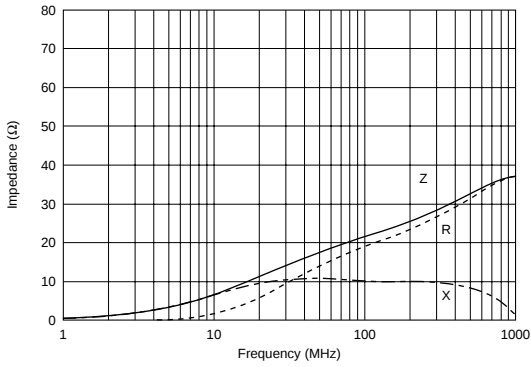
BLM03PG220SN1
