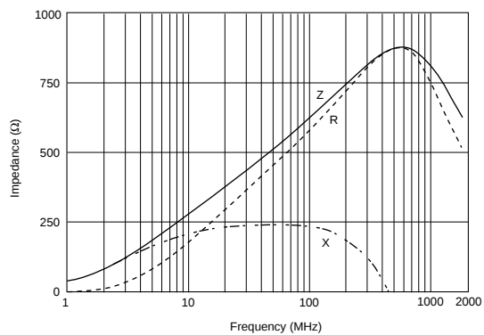
BLM18HK601SN1
