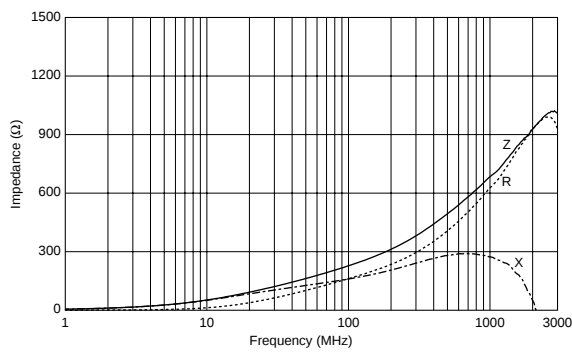
BLM15GG221SN1
