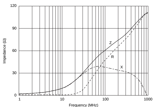
BLM15PD600SN1
