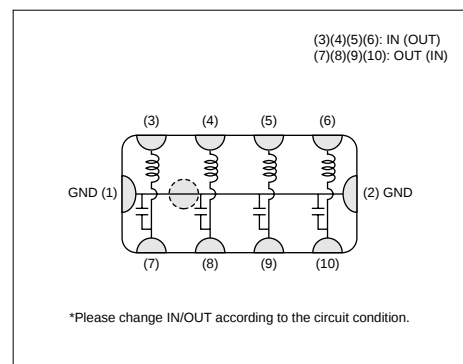
NFA18SL 307/407/487 V1A45
