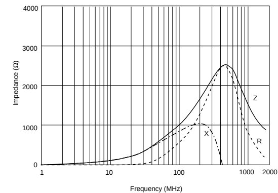
BLM18HD102SN1
