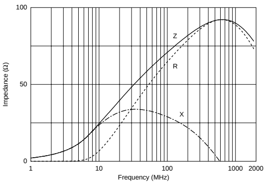
BLM18SG700TN1
