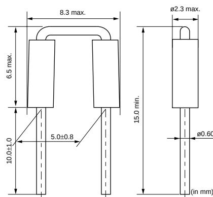
BL03RN2R1M1B
