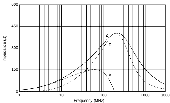
BLM18KG331SN1
