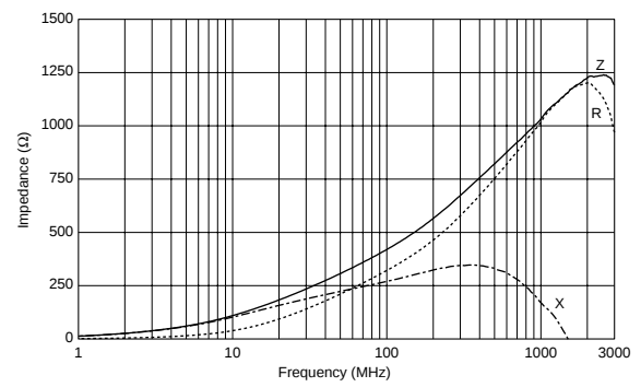
BLM15GG471SN1
