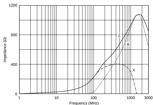
BLM15HB221SN1
