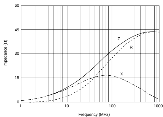
BLM31PG330SN1
