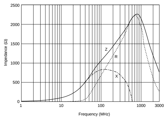
BLM15HD102SN1
