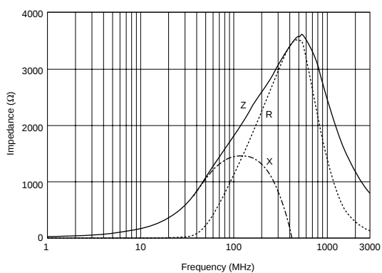
BLM15HD182SN1
