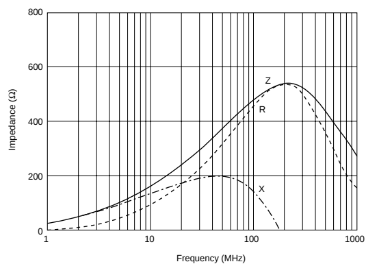
BLM18PG471SN1
