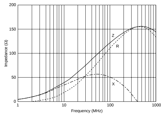
BLM18PG121SN1
