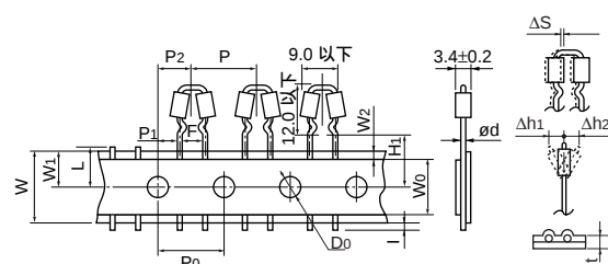
BL02RN2R3N1A
