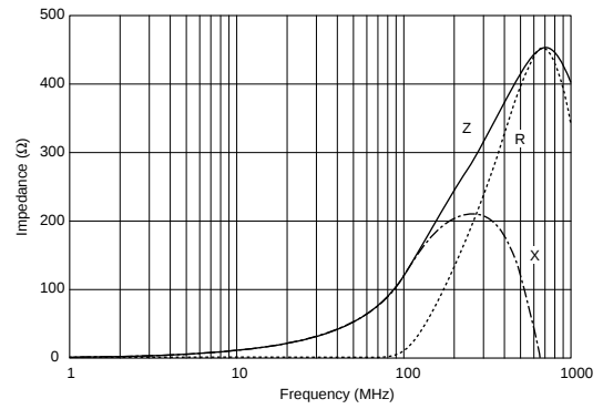
BLA2ABB121SN4
