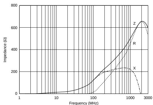
BLM15HB121SN1
