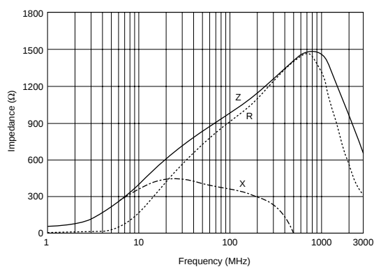
BLM15HG102SN1
