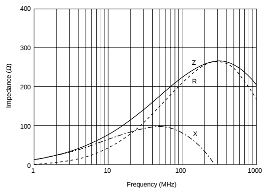
BLM18PG221SN1
