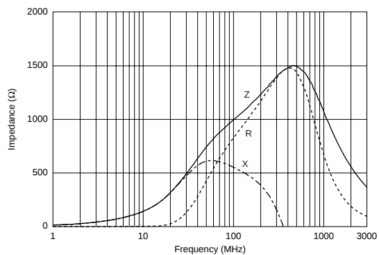
BLM18HE102SN1
