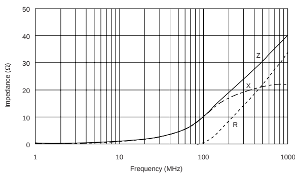
BLA2ABB100SN4
